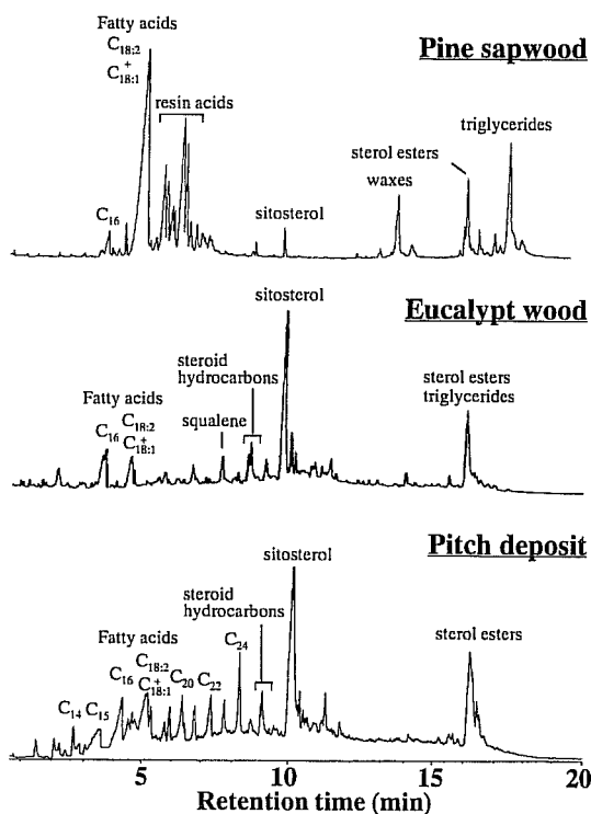
Fig. 2. GC-FID chromatograms of lipophilic extractives from pine sapwood, eucalypt wood and a pitch deposit in an eucalypt kraft pulp, obtained with the short capillary column (5 m). The oven was temperature-programmed from 100°C (1 min) to 350°C (3 min) at 15°C/min. The identity of major compounds is shown in the chromatograms.
